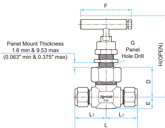
Straight Pattern
