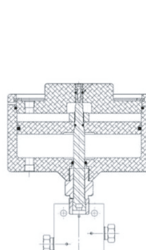
Double Acting
