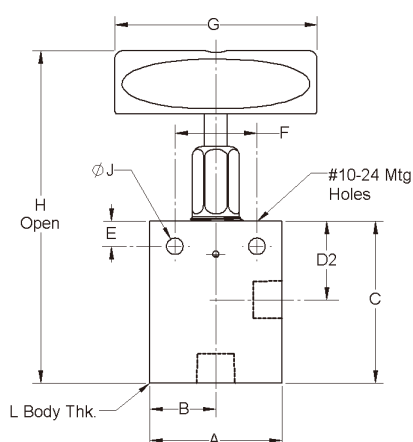
2-Way Angle
