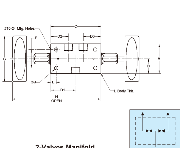
2-Valves Manifold
