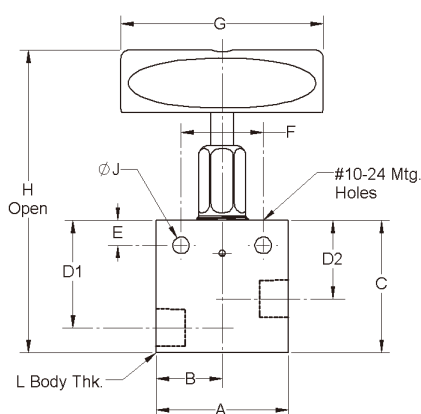
2-Way Straight
