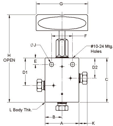
3-Way 2 Inlet
