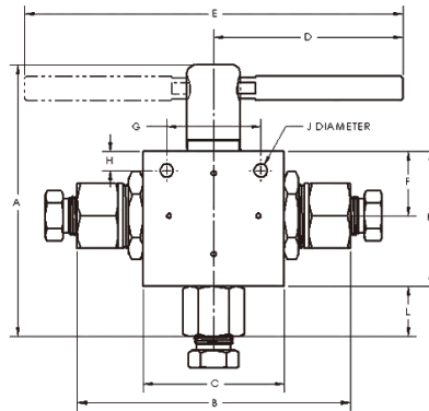
3-Way Trunnion
