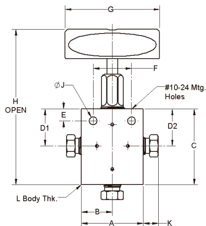
3-Way 2 Outlet
