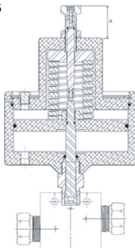
Normally Closed (Air-to-Open)
