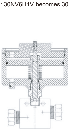
Normally Open (Air-to-Close)
