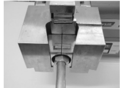
Flaring device
